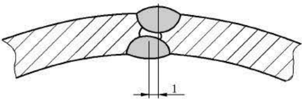
d) SAW 管焊道焊偏
